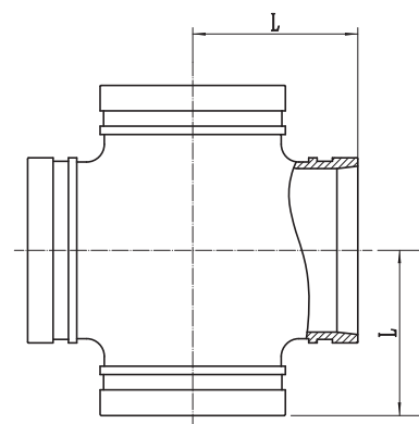
Grooved Cross Standard XGQT05
