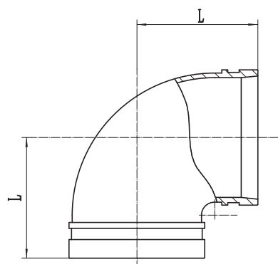
Grooved 90° Elbow Standard XGQT01L
