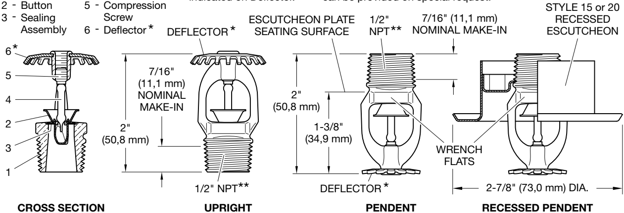
FIGURE 1 SERIES TY-FRB UPRIGHT (TY313) AND PENDENT (TY323) SPRINKLERS 5.6 K-FACTOR, 1/2 INCH NPT, QUICK RESPONSE
